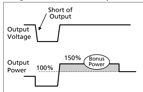
Fig. 7-5 BonusPower® after output short
