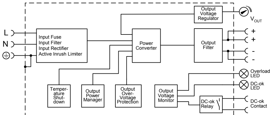
Fig. 11-1 Functional diagram
