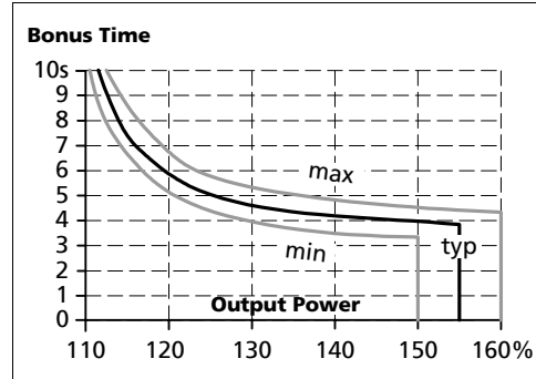
Fig. 7-2 Bonus time vs. output power
