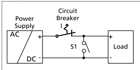
Fig. 26-5 Branch protectors, test circuit 1
