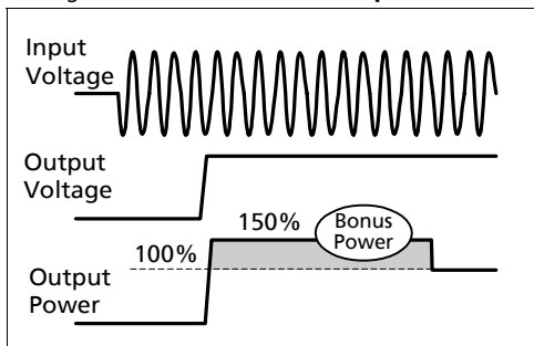
Fig. 7-4 BonusPower® after input turn-on
