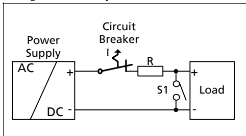
Fig. 26-6 Branch protectors, test circuit 2
