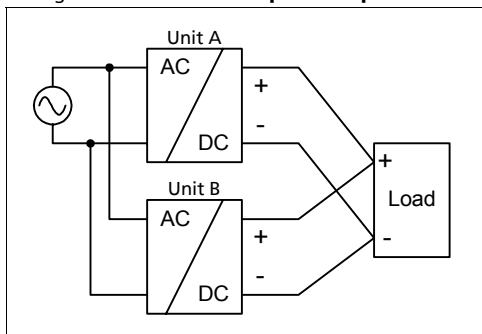
Fig. 26-7 Schematic for parallel operation
